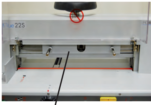
Blade change safety tool in place
