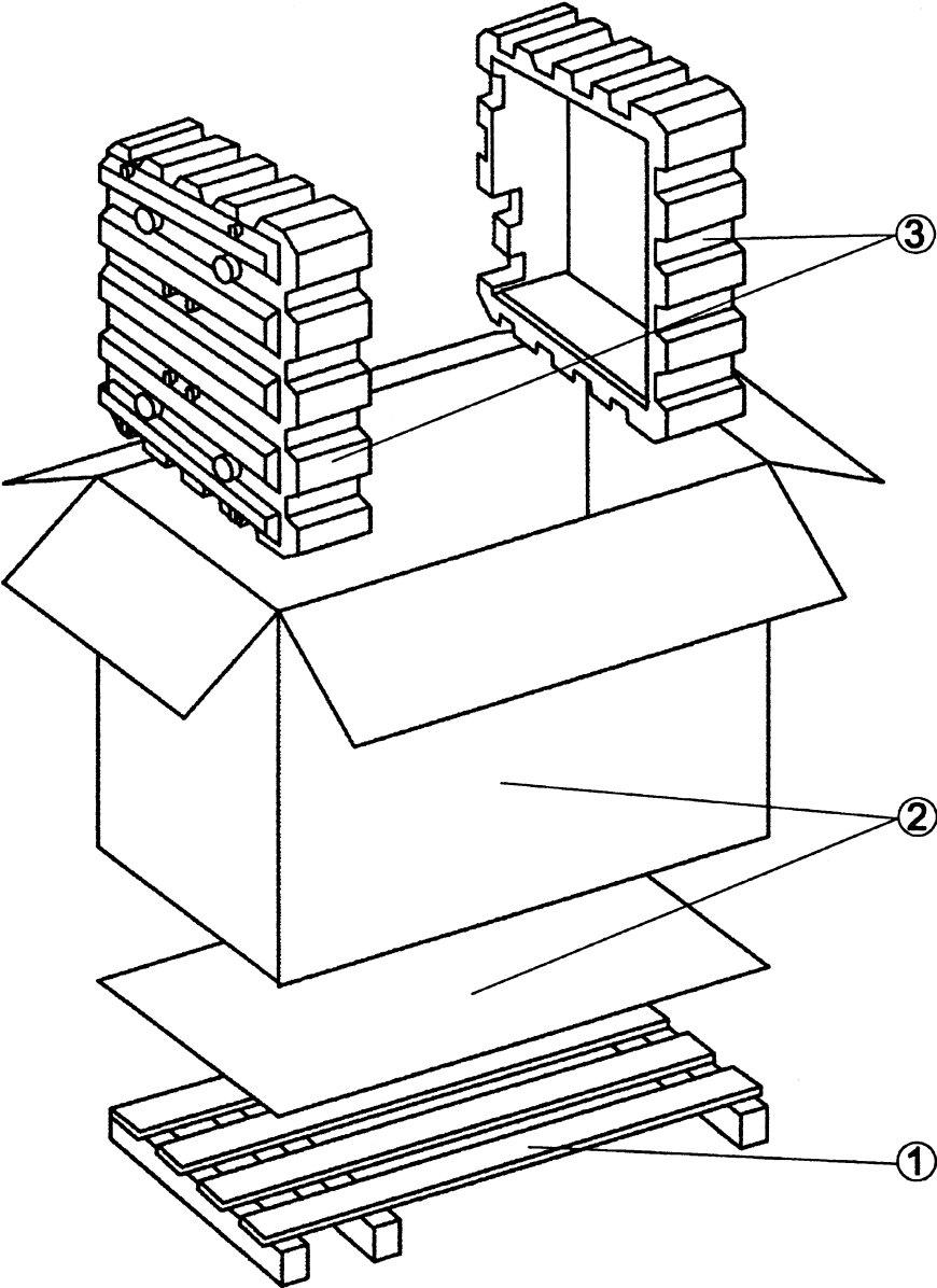
Section 8.0 2020CC Parts List Packaging Exploded View Figure 8.4
