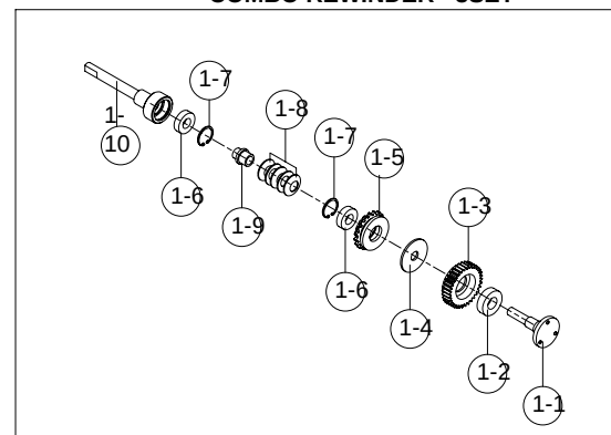
COMBO REWINDER - 3SET
