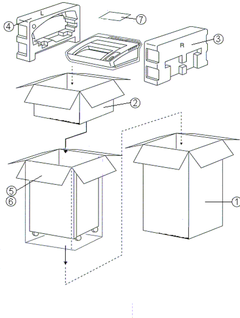
Section 8.0 4220S/4230S/4260X. Parts List 4220S/4230S/4260X. Packaging Exploded View Figure 8. 8
